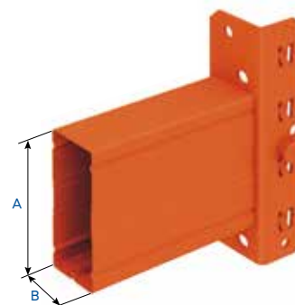
Belka TB (100, 120, 130)
